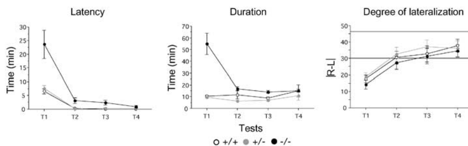
Figure 3 Latency, duration, and degree of lateralization of ambidextrous ( |R-L| \leq 30 ) mice as measured in a test-retest experiment with WT (+/+), HT (+/-), and KO (-/-) mice of the B6-DAT strain ( n = 15-16 mice per group). Horizontal lines in the right-handed panel indicate the criteria defining high ( |R-L| \geq 46 ) and low ( |R-L| \leq 30 ) lateralization scores. ANOVA for the latency: genotype, F_{2,176} = 16.8 , P < 0.0001 ; test, F_{3,176} = 42.7 , P < 0.0001 ; and interaction F_{6,176} = 7.36 , P < 0.0001 ; for the duration: genotype, F_{2,176} = 27.1 , P < 0.0001 ; test, F_{3,176} = 11.9 , P < 0.0001 ; and interaction F_{6,176} = 11.2 , P < 0.0001 . Data points depict mean \pm SEM.
